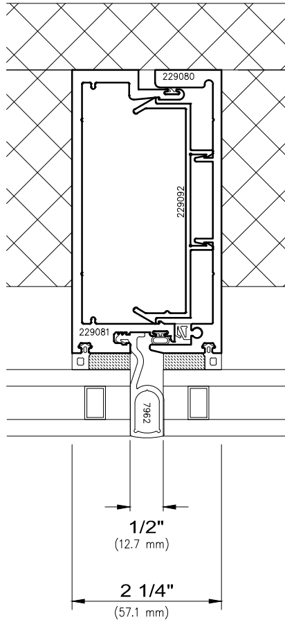
9 Spandrel/Spandrel Mullion Stack
